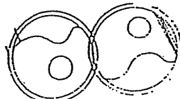
Chlorella
